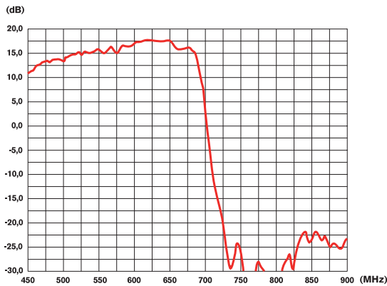
Diamond gain curve
